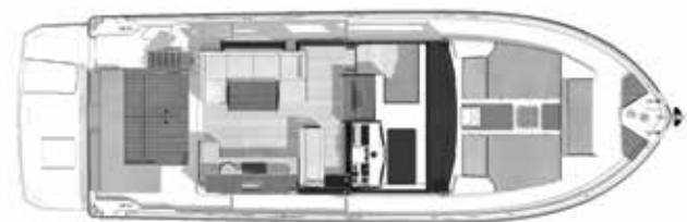
MAIN DECK + BOW DECK + AFT TERRACE
